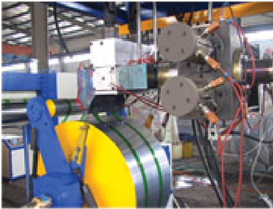
Extruded Rough Strip Casting
